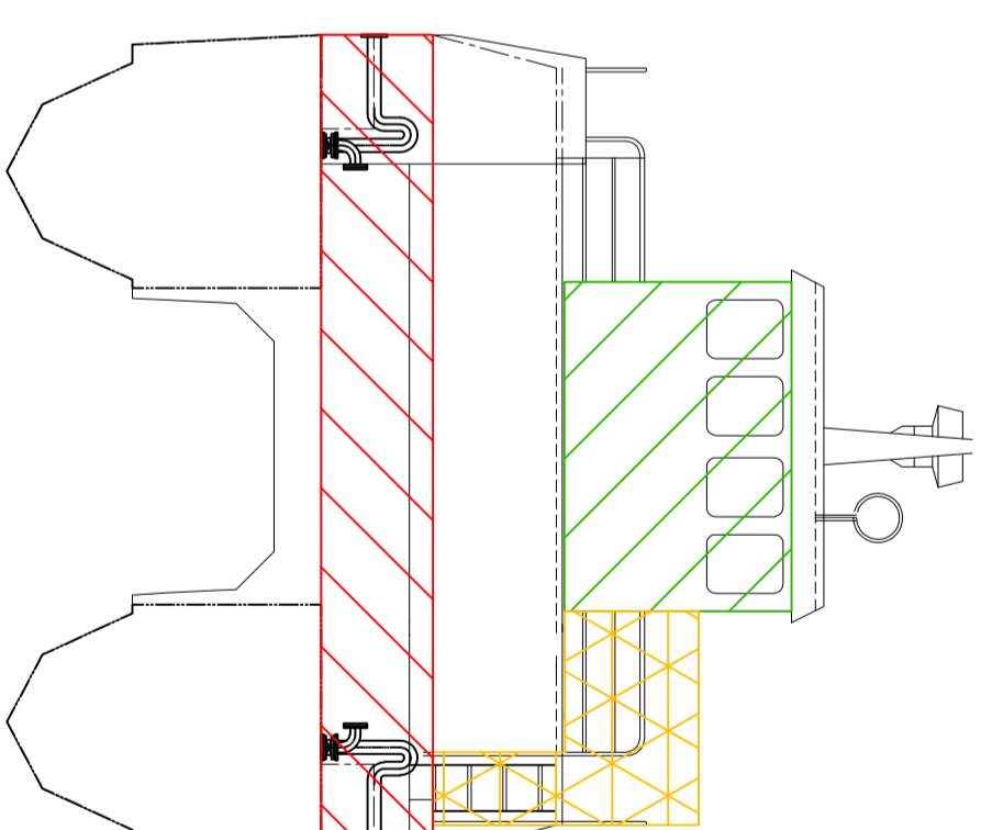
SECTION VIEW
