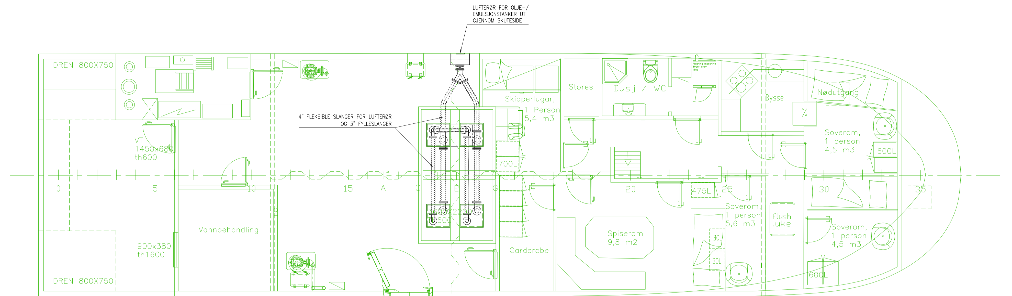
HV-DECK
