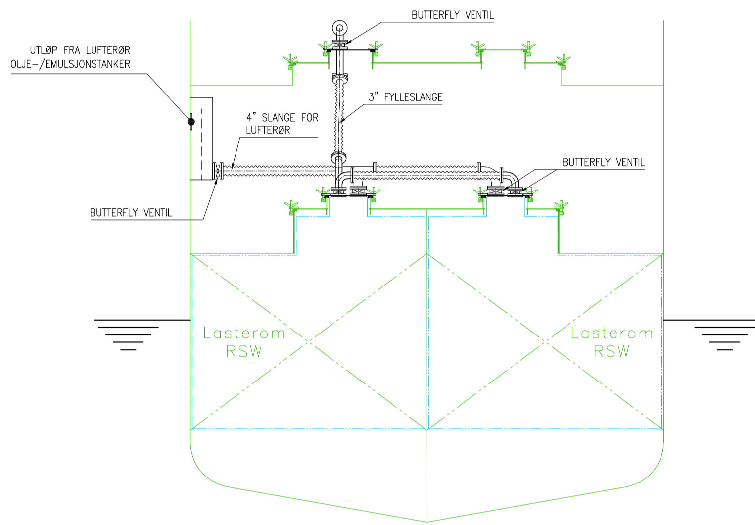
SECTION ~#C-G
